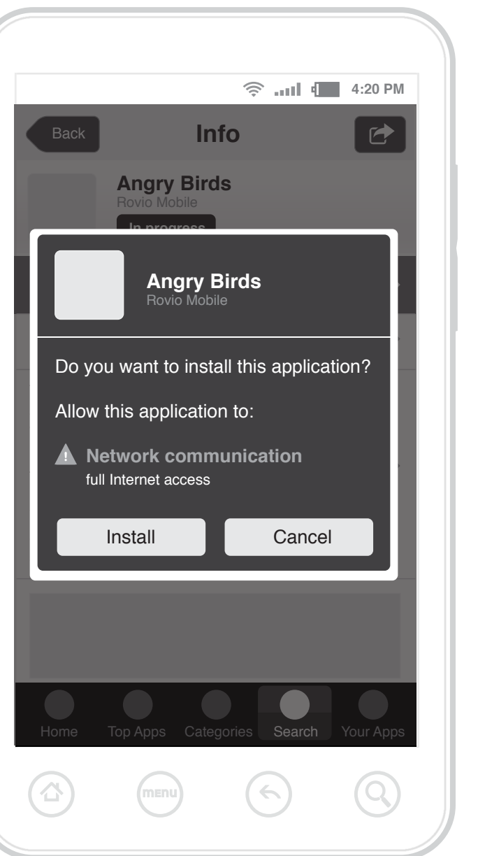
4.4 Installation Confirmation
