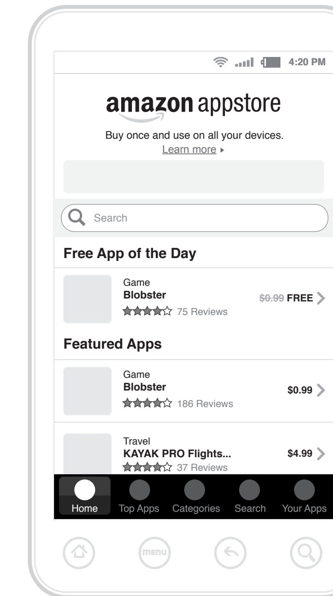
1.0 Home
