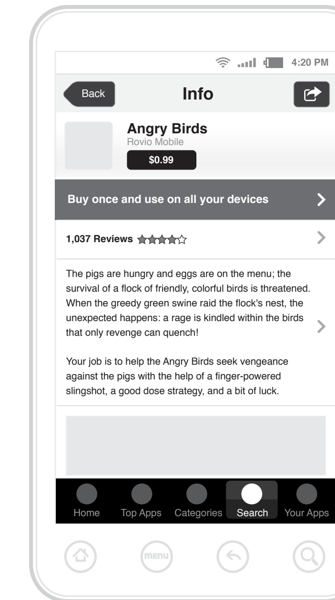
4.0 Detail Page
