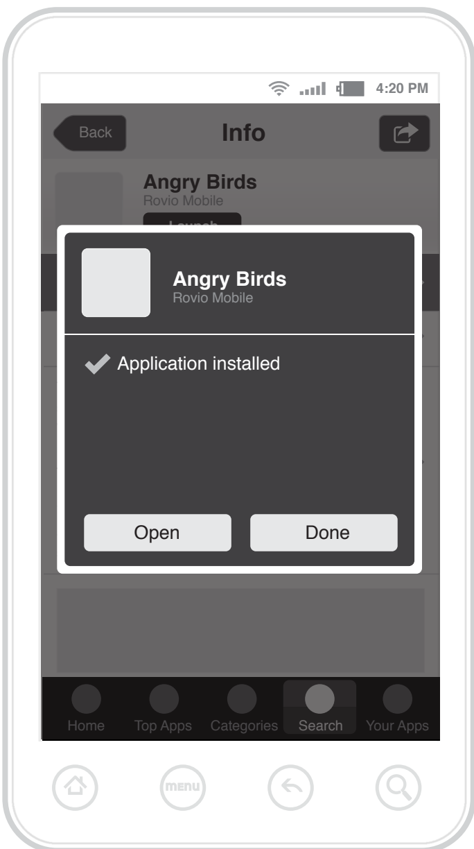
4.5 Installation Complete
