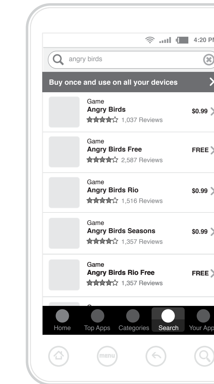
2.0 Search
