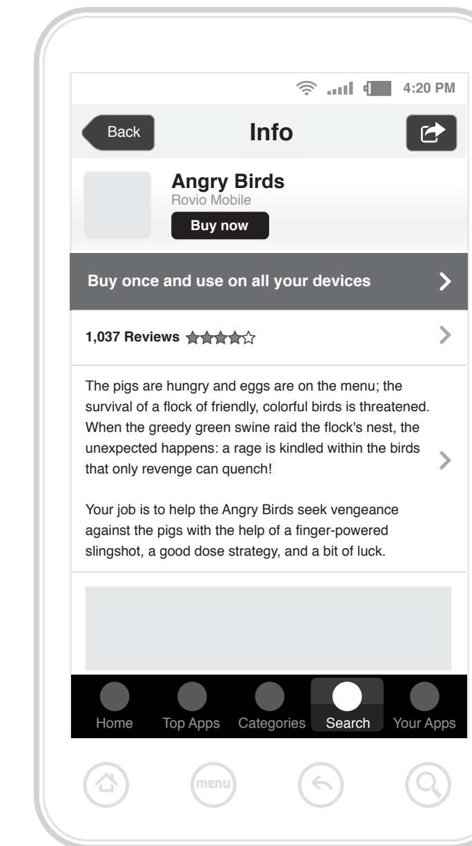
4.1 Purchase Confirmation
