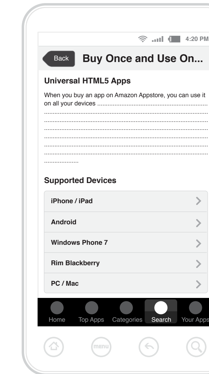
3.0 Entitlement Info
